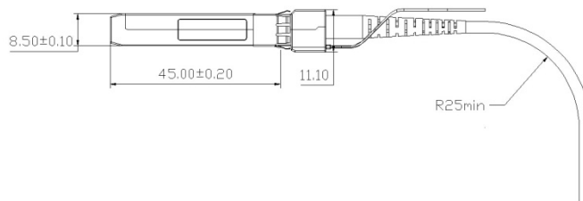
SFP+ AOC end Mechanical Specifications
